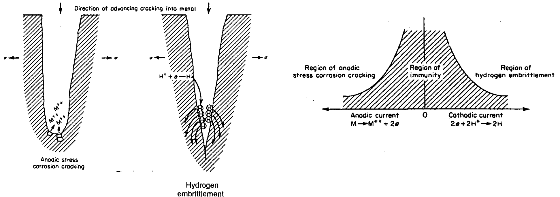
Schematic differentiation of anodic cracking and cathodically sensitive embrittlement.
